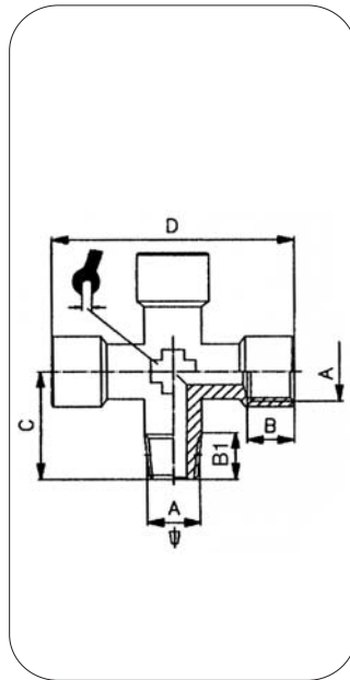
ART. 120 Croce M.F.F. 1 male 3 female cross
