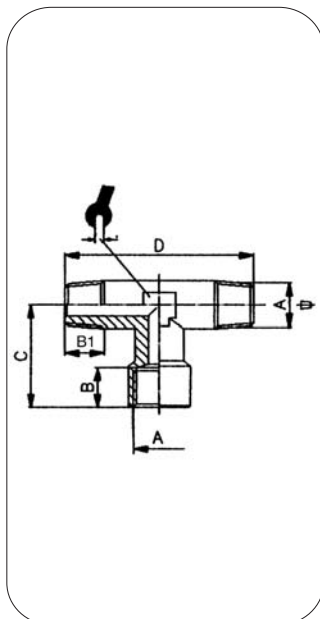
ART. 117 T.M.F.M. Centre female tee
