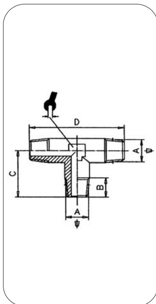
ART. 116 T.M.M. Male tee
