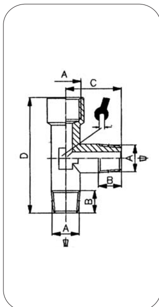
ART. 118 T.M.F.F. Off-set female tee
