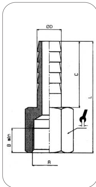
ART. 122 Portagomma femmina Female Hose adapter
