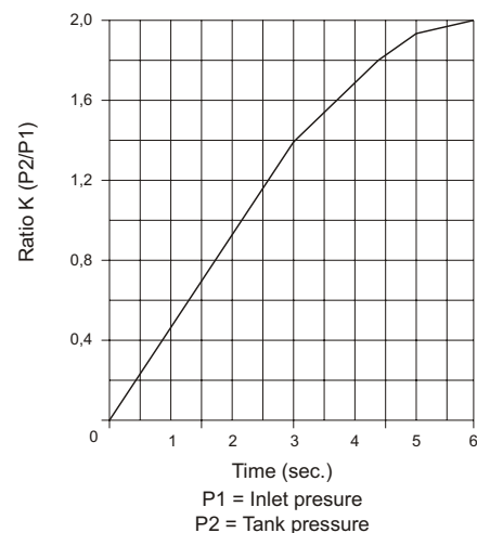
Filling time curve 10 liters tank
