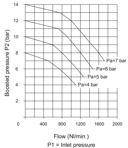
Flow rate curves
