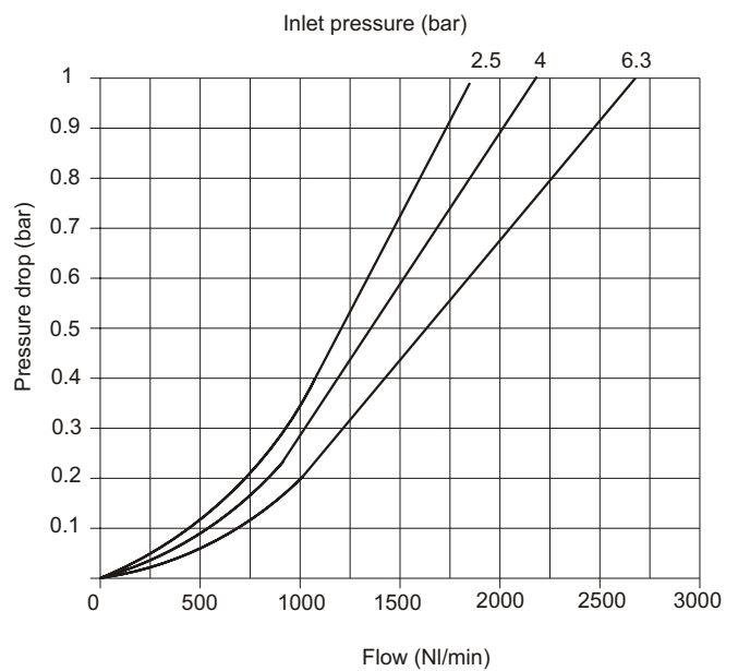
Flow rate curves
